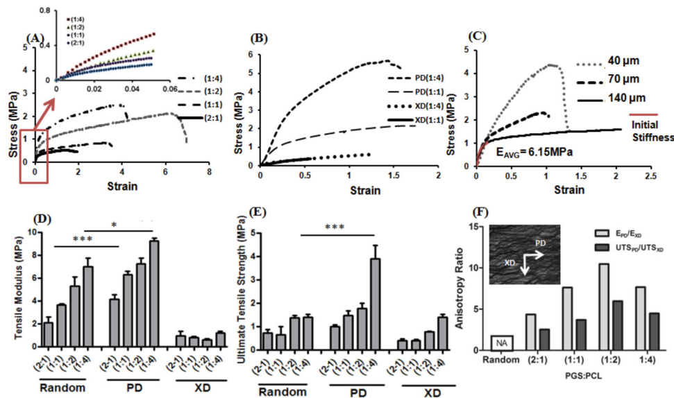
Figure 3. Uniaxial mechanical testing of unseeded scaffolds in two directions. A) Representative stress–strain curves of random scaffolds for all the ratios of the PGS:PCL scaffolds demonstrated that scaffolds with random fibers deformed extensively following 5%–10% strain. The initial stiffness and UTS increased by increasing the PCL content in polymer ratios. B) Representative stress–strain curves of aligned scaffolds for (1:1) and (1:4) ratios of the PGS:PCL shown in two directions (PD and XD). Scaffolds were stiffer in PD directions. C) Representative stress–strain curves of aligned scaffolds with different thicknesses depicted for the ratio of (2:1). Similar initial stiffnesses were observed with divergent relationships between UTS and scaffolds stiffness. As the thickness of the aligned scaffolds increased, greater deformations were observed in the stress–strain curves. This deformation was similar to that of the random fiber scaffolds. D,E) Tensile modulus and UTS were compared between random and aligned scaffolds in PD and XD direction. F) Anisotropy of scaffolds was measured for PGS:PCL scaffolds of varying ratios, which demonstrated that the values for (1:1), (1:2), and (1:4) were similar to the native tissues.
